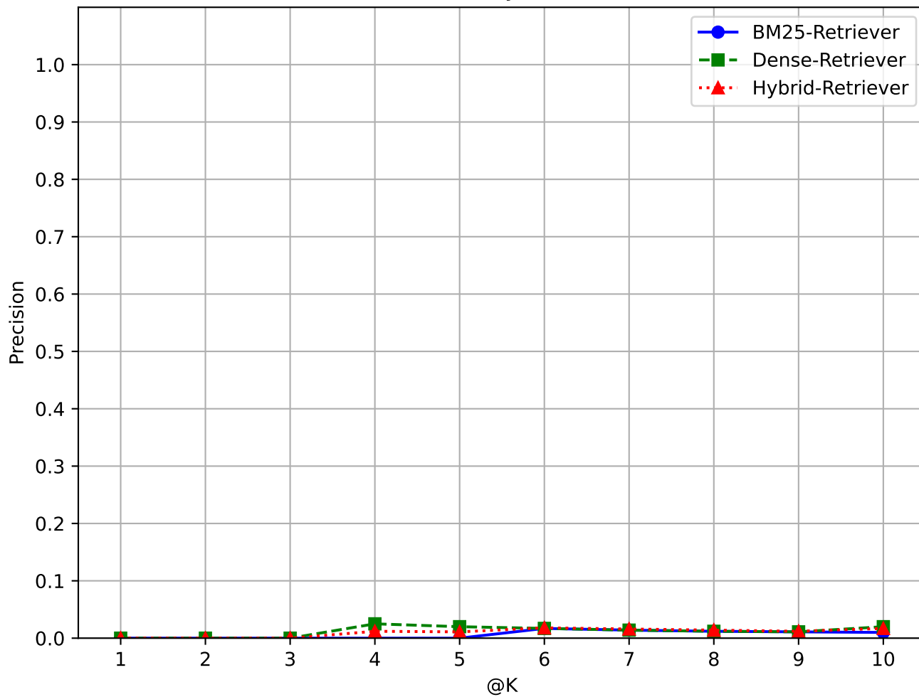
Query 38
